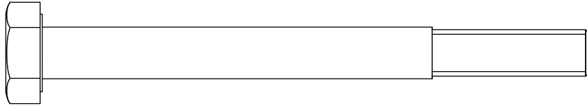
E1. M10x110 Hex Head Bolt (Partial Thread) Qty. 2
