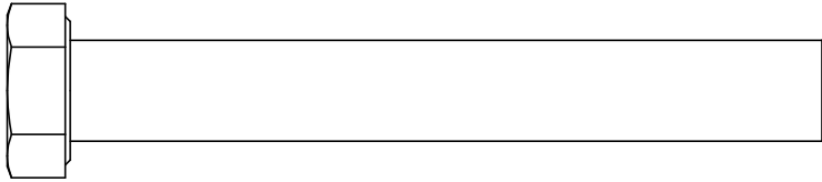
Part #2 HEX HEAD BOLT M10X65mm
