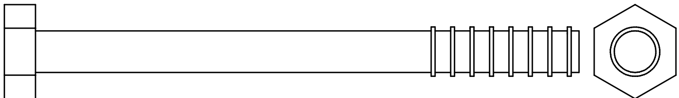
(A5)HEX BOLT 1/2"x5 1/2"L PARTIAL THREAD QTY.3
